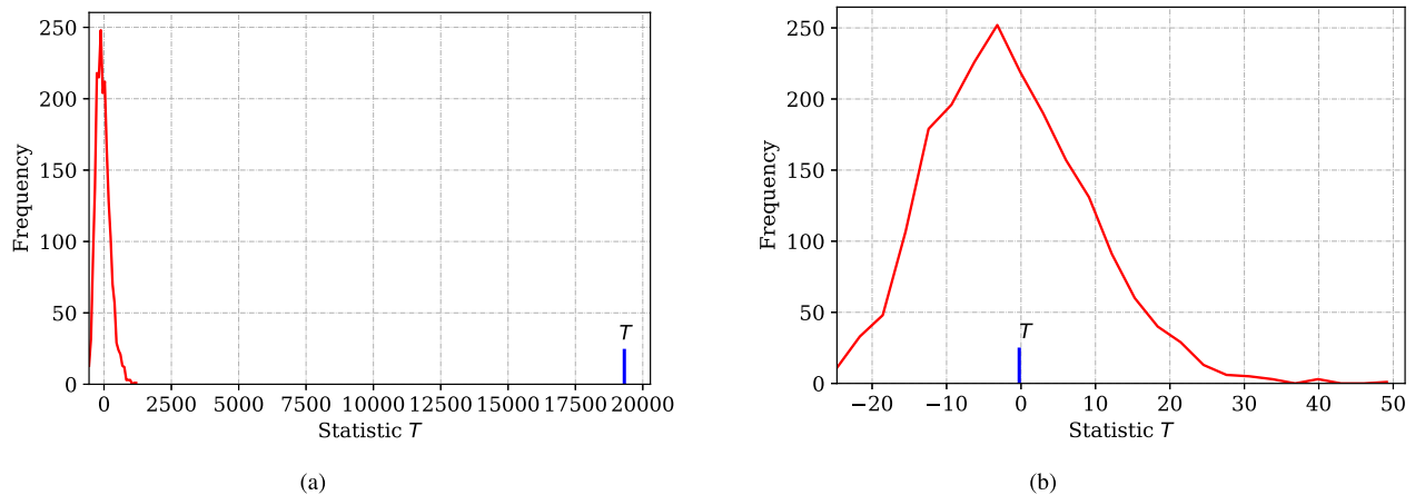
Fig. 3. Computed statistic T , with \rho = 5 and \gamma = 1.0 , in comparison to the distribution computed from the Monte Carlo simulation. (a) Case I. (b) Case II.
